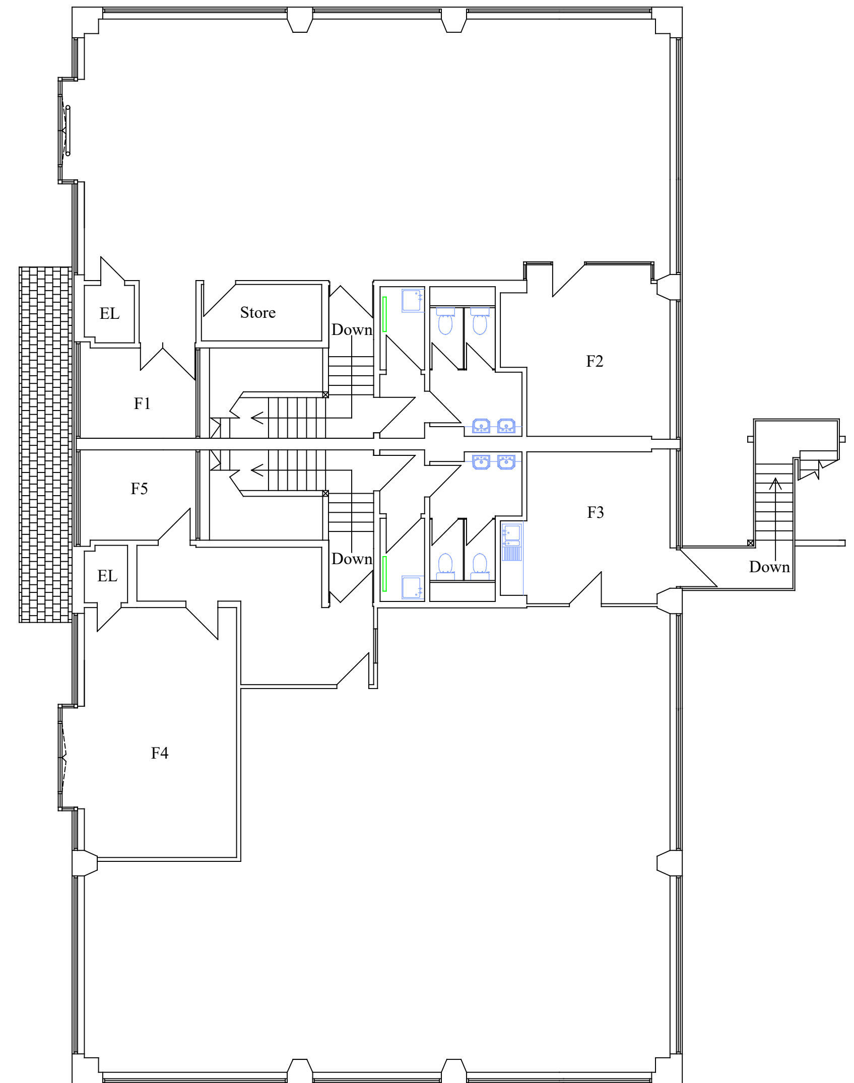
FIRST FLOOR
