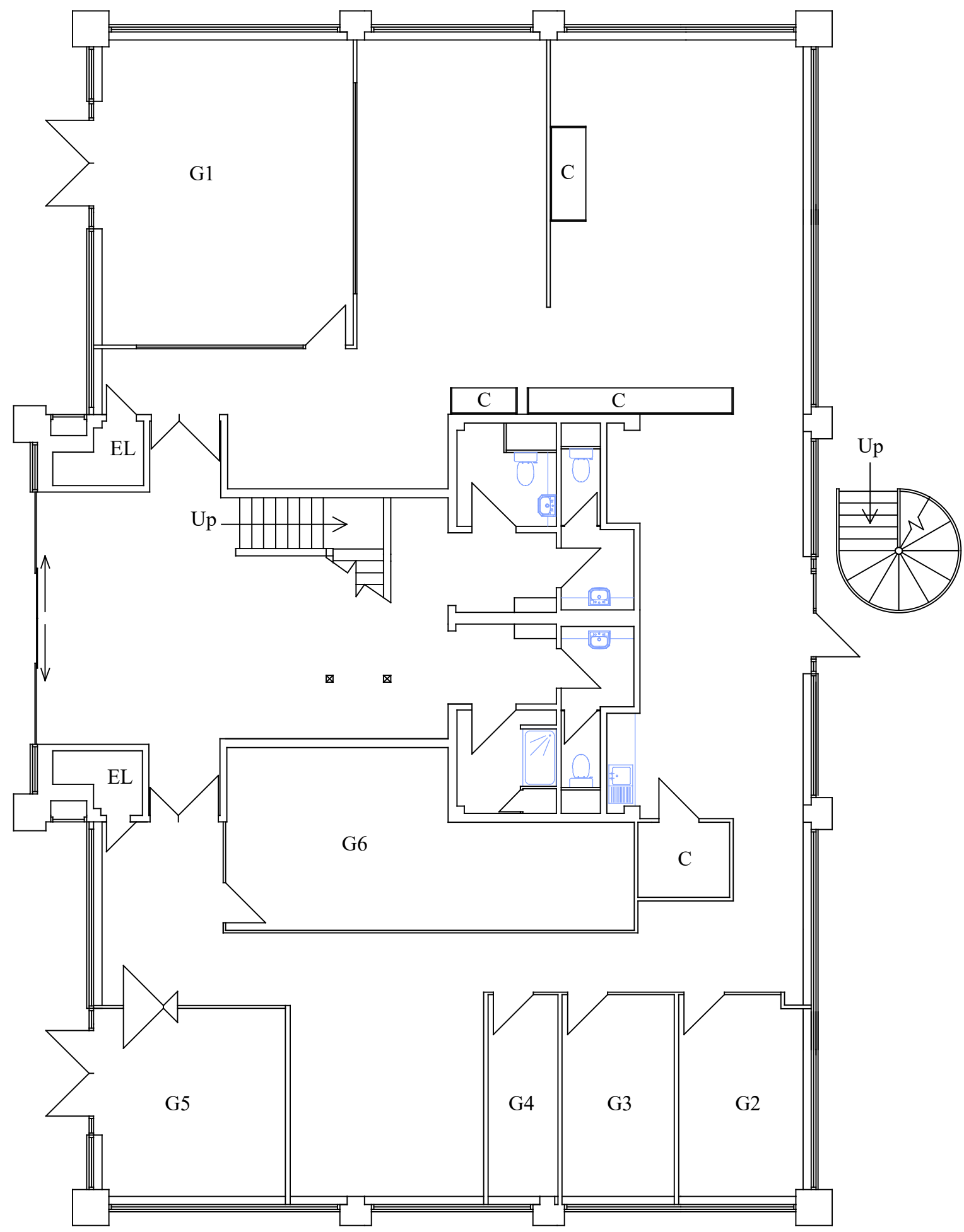
GROUND FLOOR
