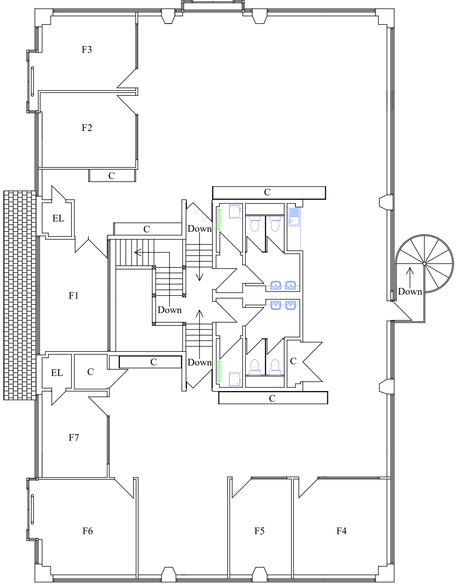
FIRST FLOOR
